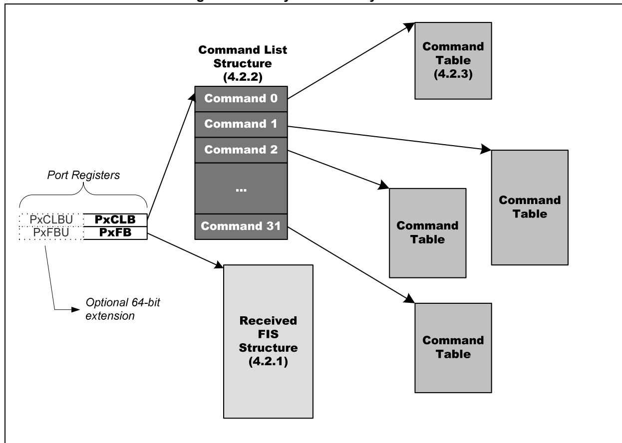
Figure 5: Port System Memory Structures
