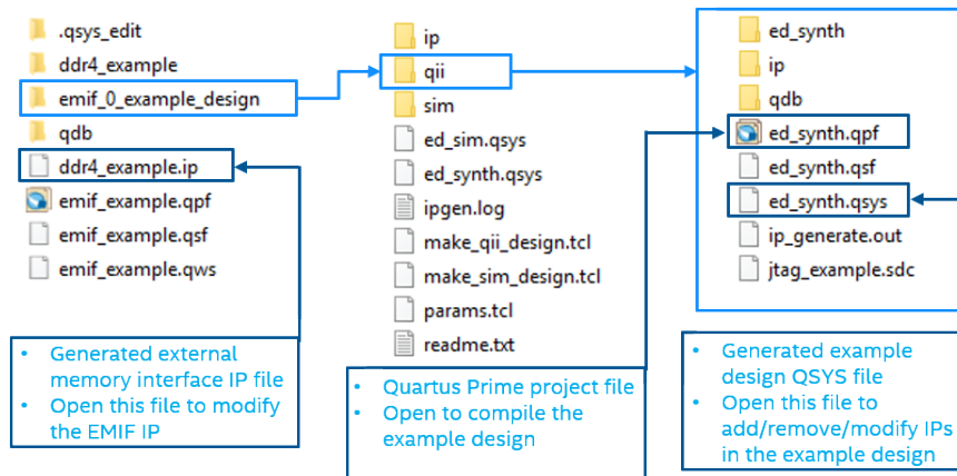
Figure 3. Generated Synthesizable Design Example File Structure
