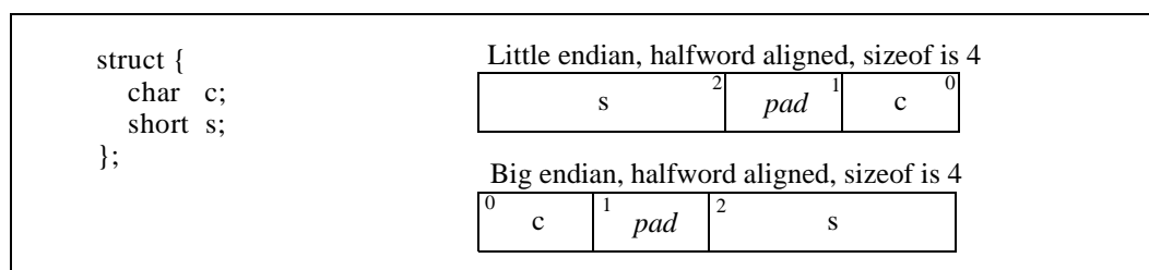
Figure 4-3. Internal Padding
